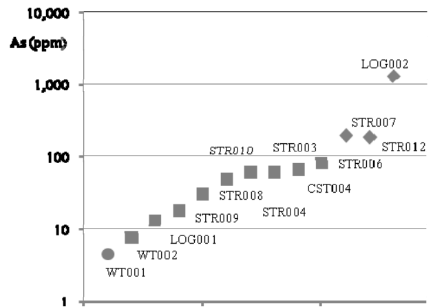
Figure 2: Arsenic content of waste slurries.
