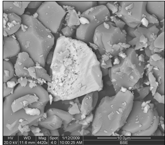
Figure 1: SEM photomicrograph of alumina lapping slurry with smaller GaAs fragments.
