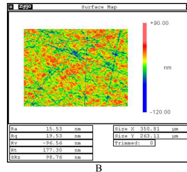
FIGURE 10 SURFACE FINISH AFTER LAPPING C-PLANE SAPPHIRE: A) EXISTING COMMERCIAL PRODUCT, B) NOVEL SLURRY DEVELOPED BY ENGIS
