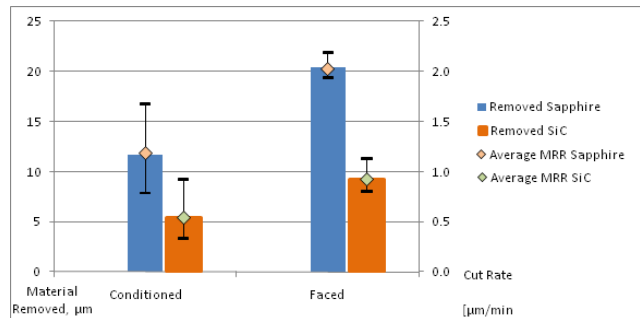
FIGURE 5 EFFECT OF PLATE TEXTURE ON REMOVAL RATE OF SAPPHIRE AND SILICON CARBIDE
