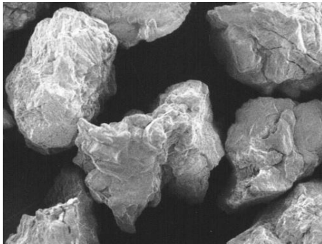
FIGURE 7 MICROGRAPH OF PC DIAMOND
