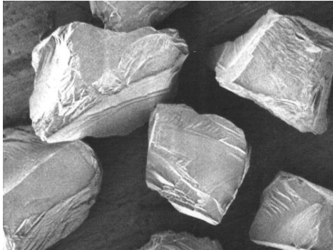
FIGURE 6 MICROGRAPH OF MA DIAMOND
