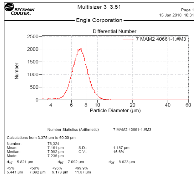
FIGURE 2 DIAMOND PARTICLE SIZE DISTRIBUTION
