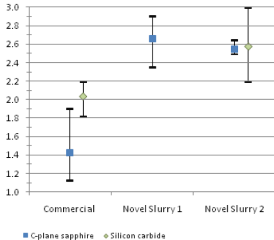
FIGURE 9 CUT RATE RESULTS FOR RAPID LAPPING OF SAPPHIRE AND SILICON CARBIDE.
