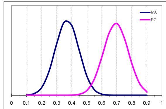
FIGURE 8 CUT RATE COMPARISON FOR LAPPING R-PLANE SAPPHIRE USING 3µm DIAMOND ON HY-CU PLATE, DIAMOND TYPE MA VS. PC.
